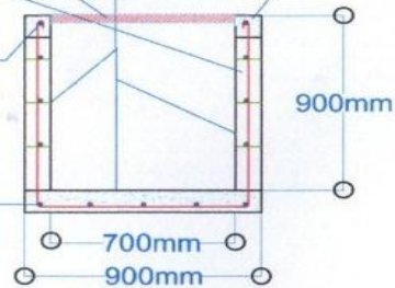
MANHOLE DETAIL SCALE 1:20M
