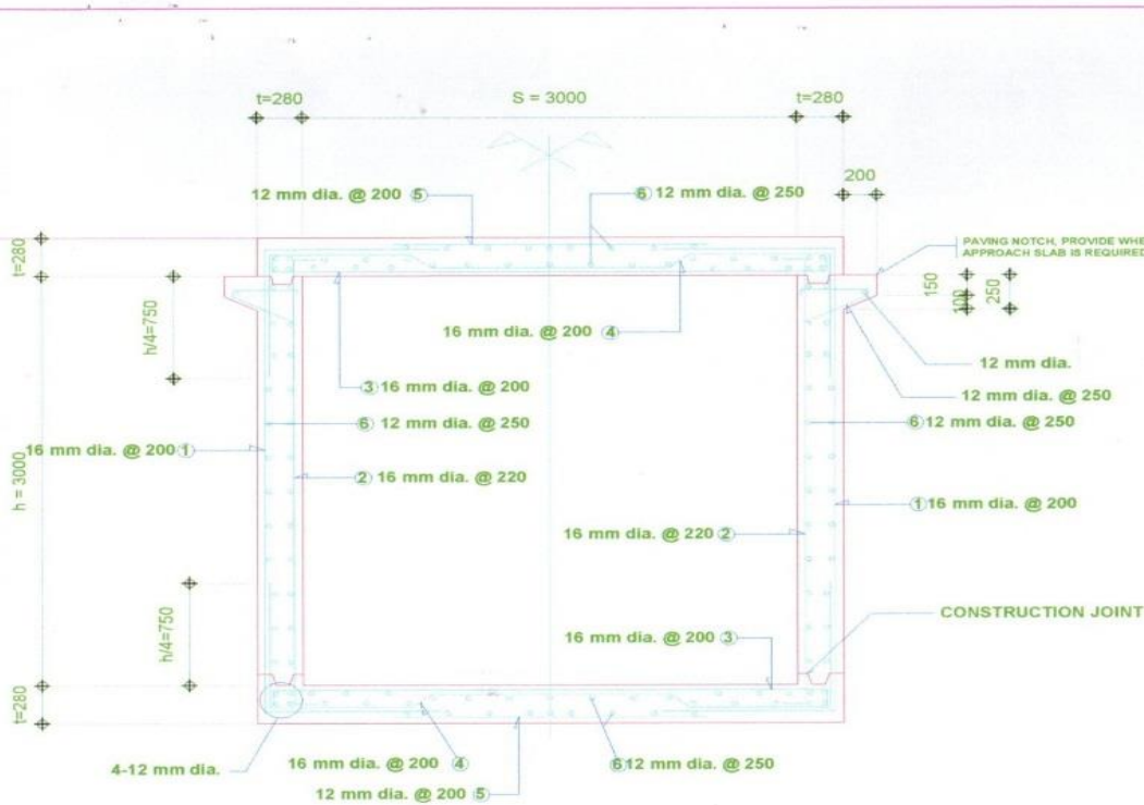
SECTION - SINGLE BARREL NTS
