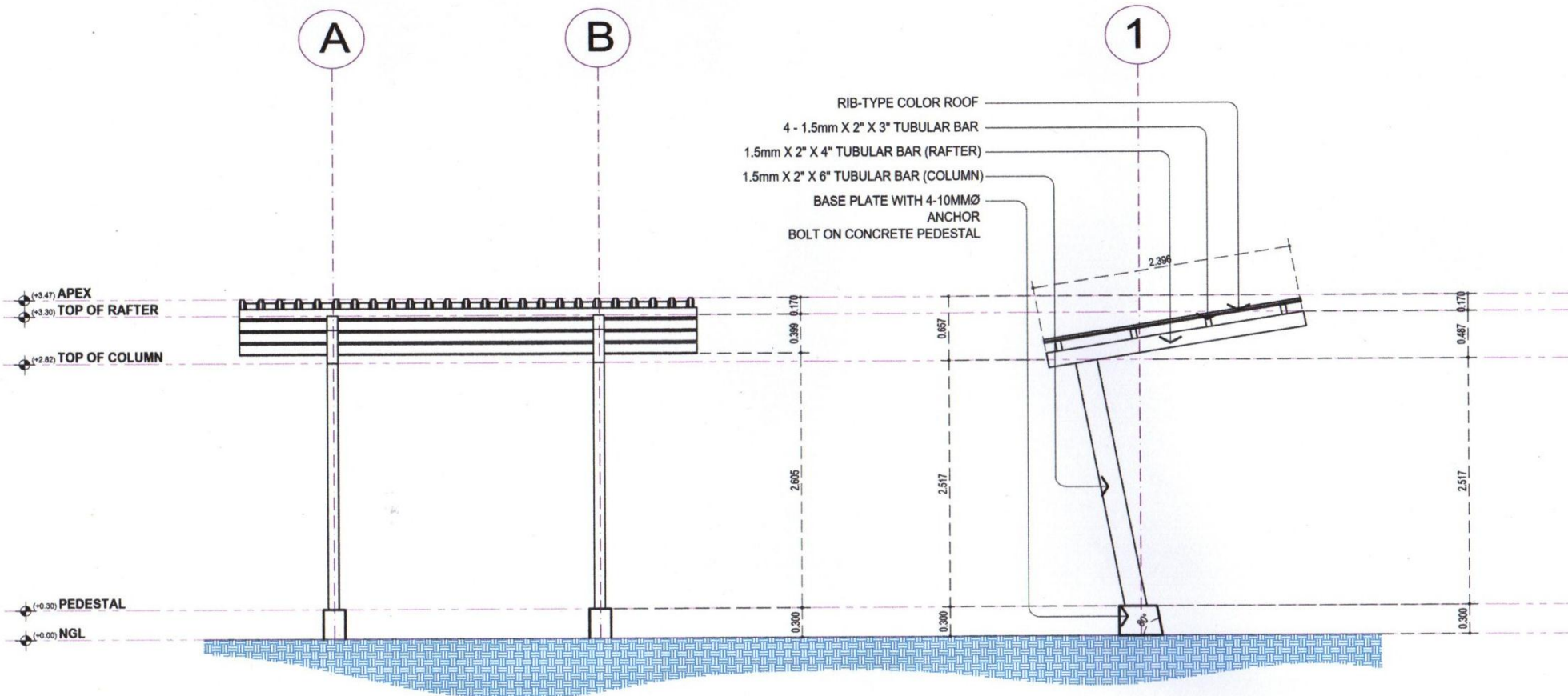
SHED ROOF FRONT ELEVATION SCALE 1:50 MTS.
