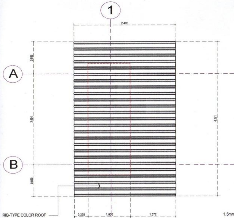
SHED ROOF ROOF PLAN SCALE 1:40 MTS.
