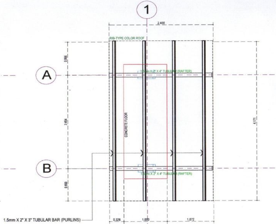
SHED ROOF ROOF FRAMING PLAN SCALE 1:40 MTS.
