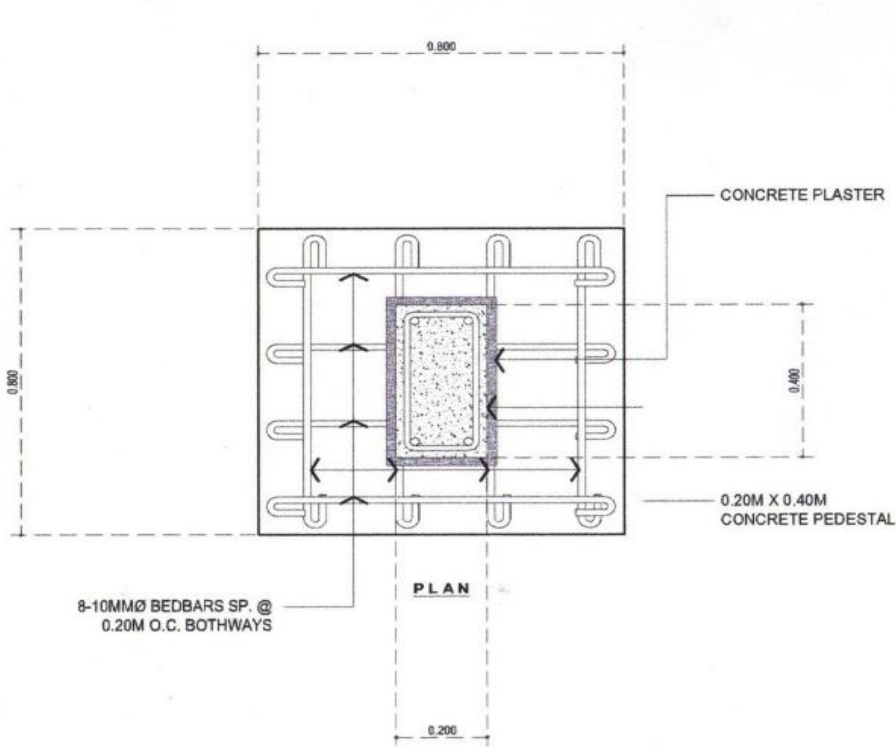
SHED ROOF CONCRETE PEDESTAL DETAIL SCALE 1:15 MTS.
